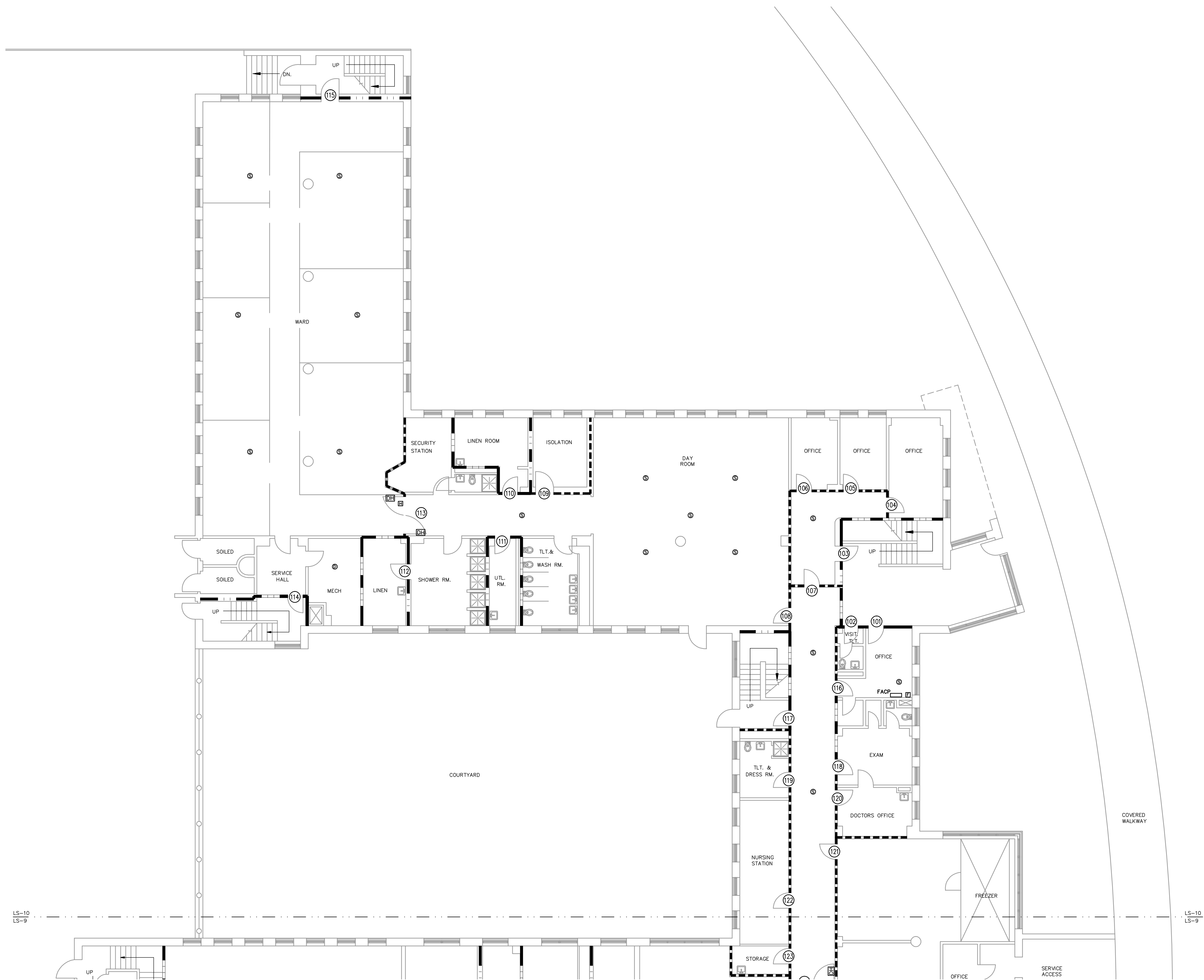
OAKCREST HOUSE FIRST FLOOR - WEST SCALE: 3/32" = 1'-0"
