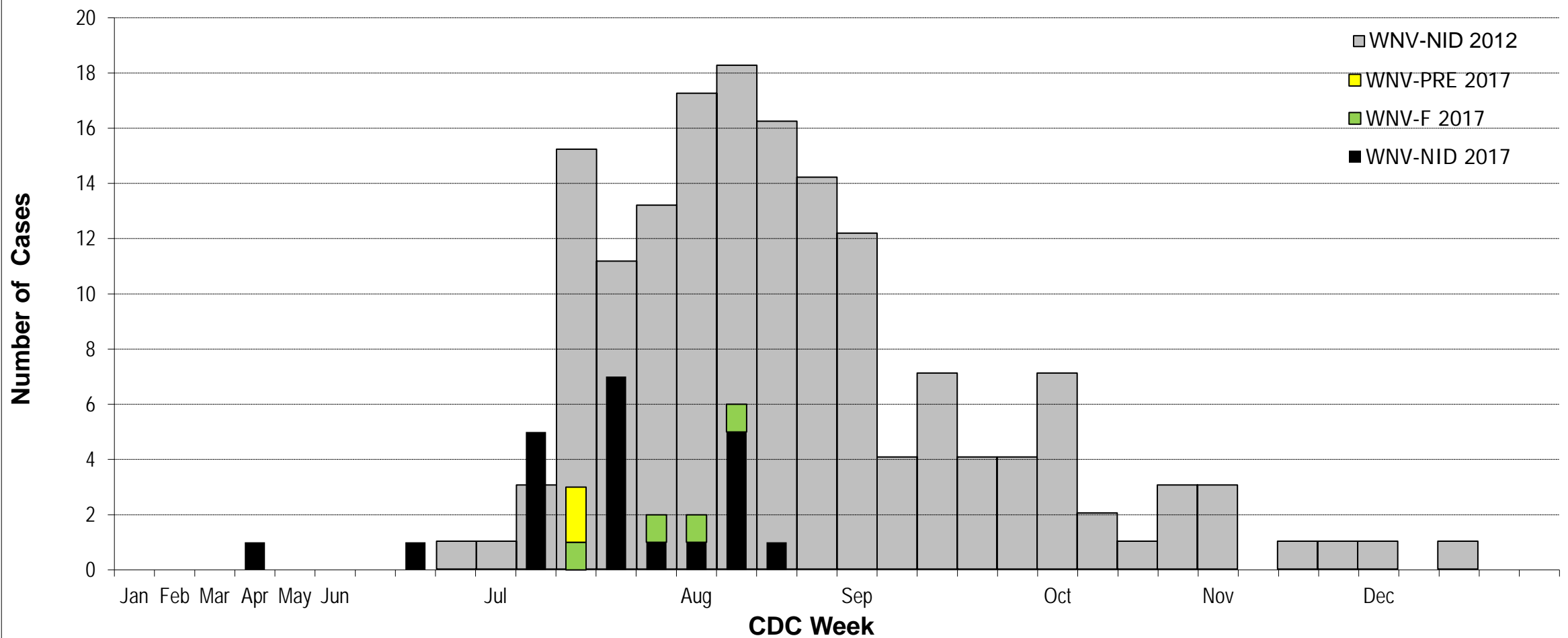
WNV Cases - Louisiana, 2012 compared to 2017
